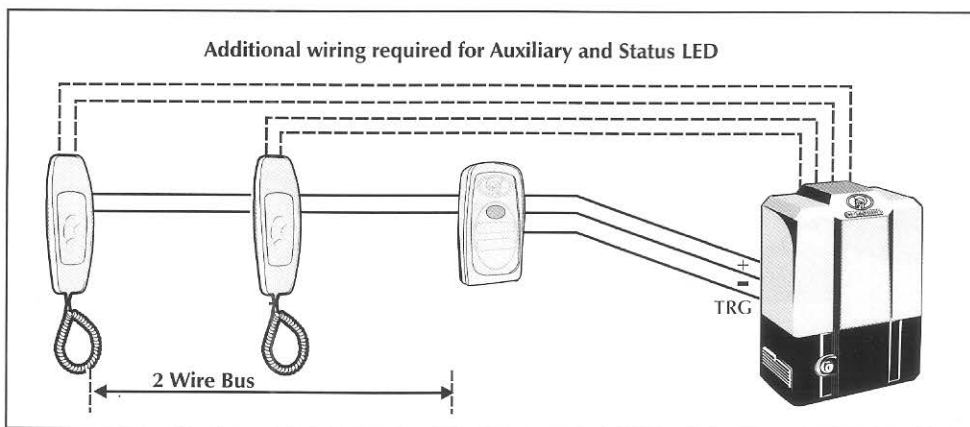
Fig 2 Wiring Requirements
